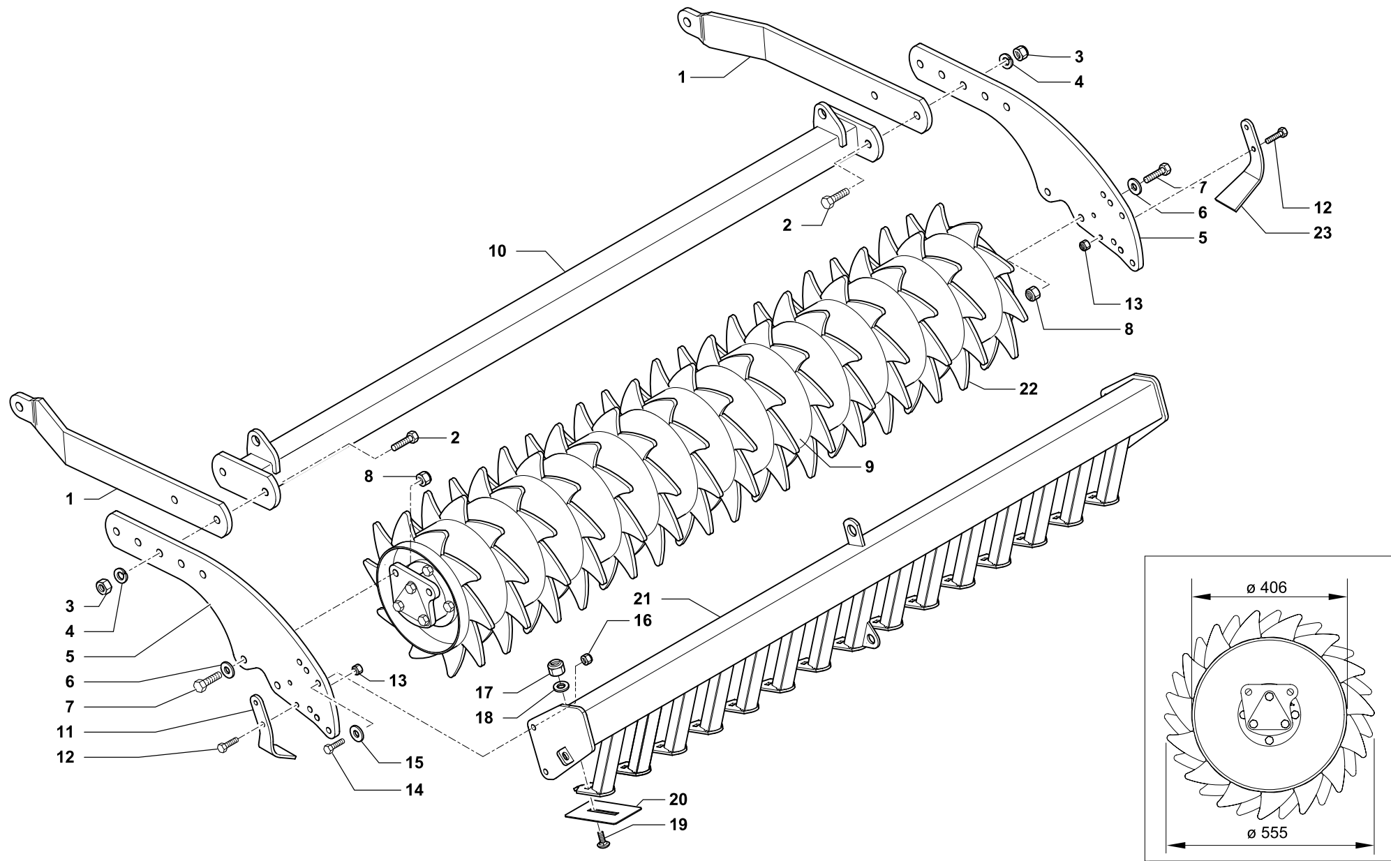
PACKER ROLLER Ø 555
