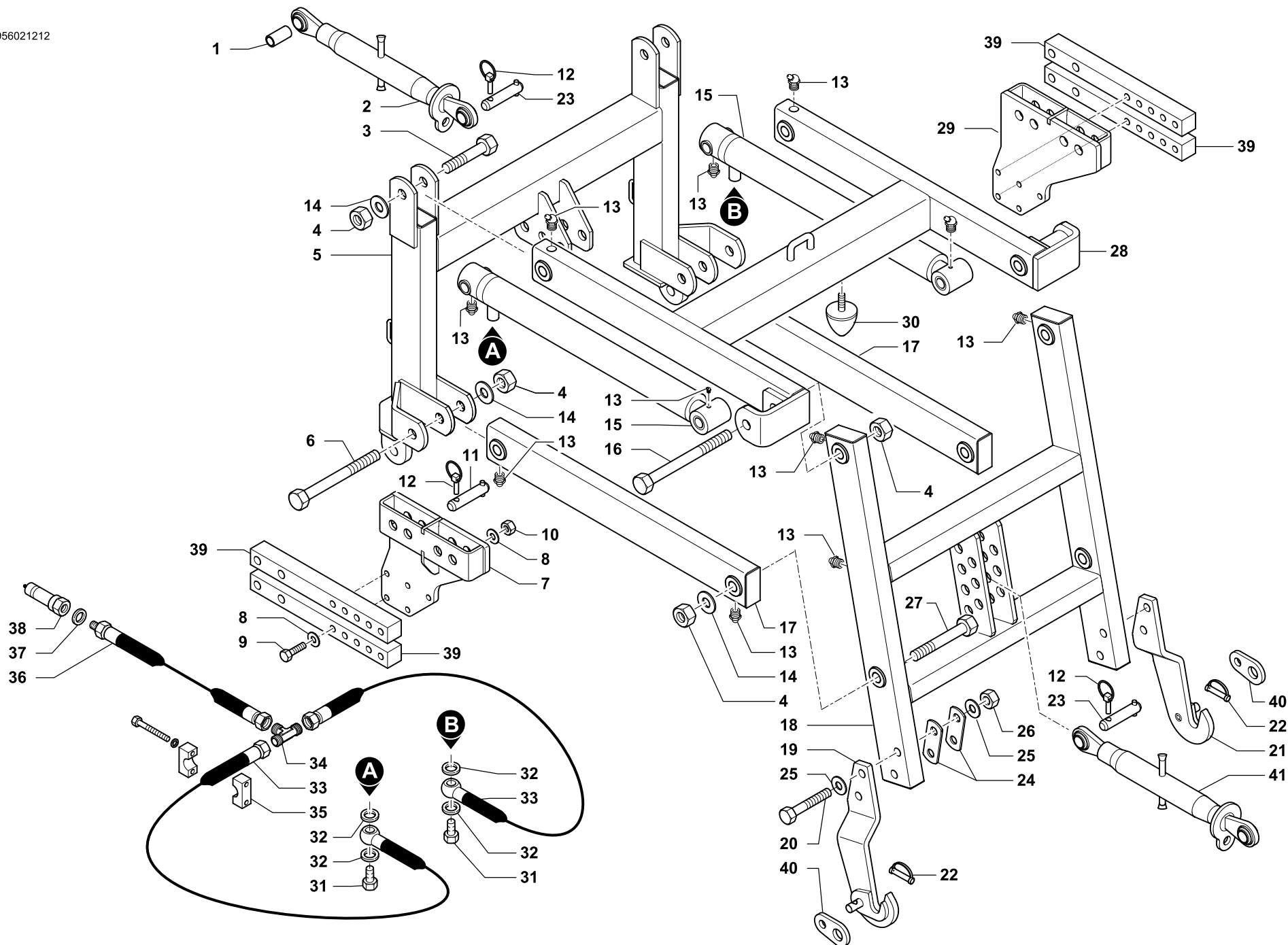
HYDRAULIC SEEDING MACHINE HITCH "TWIN"
