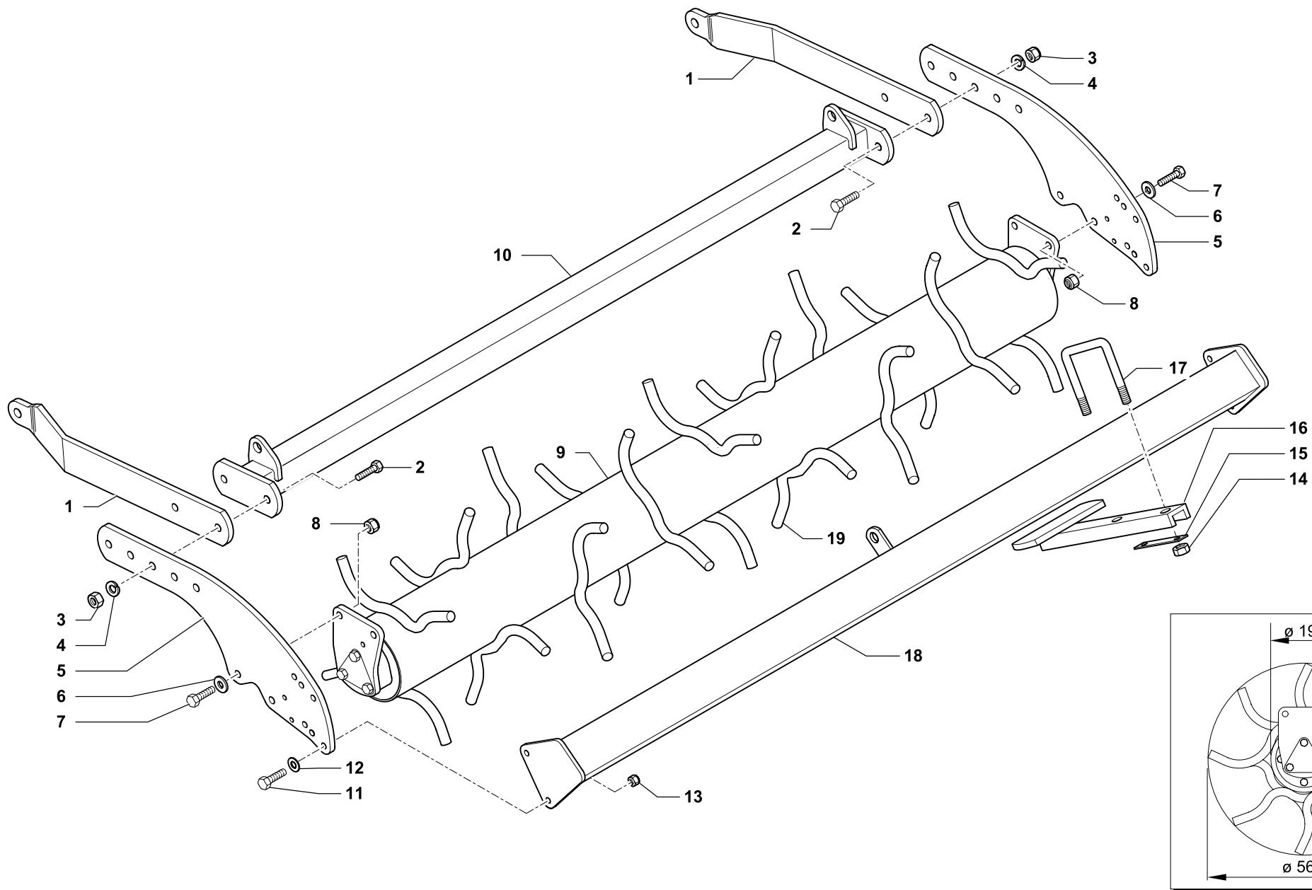
SPIKES ROLLER Ø 560
