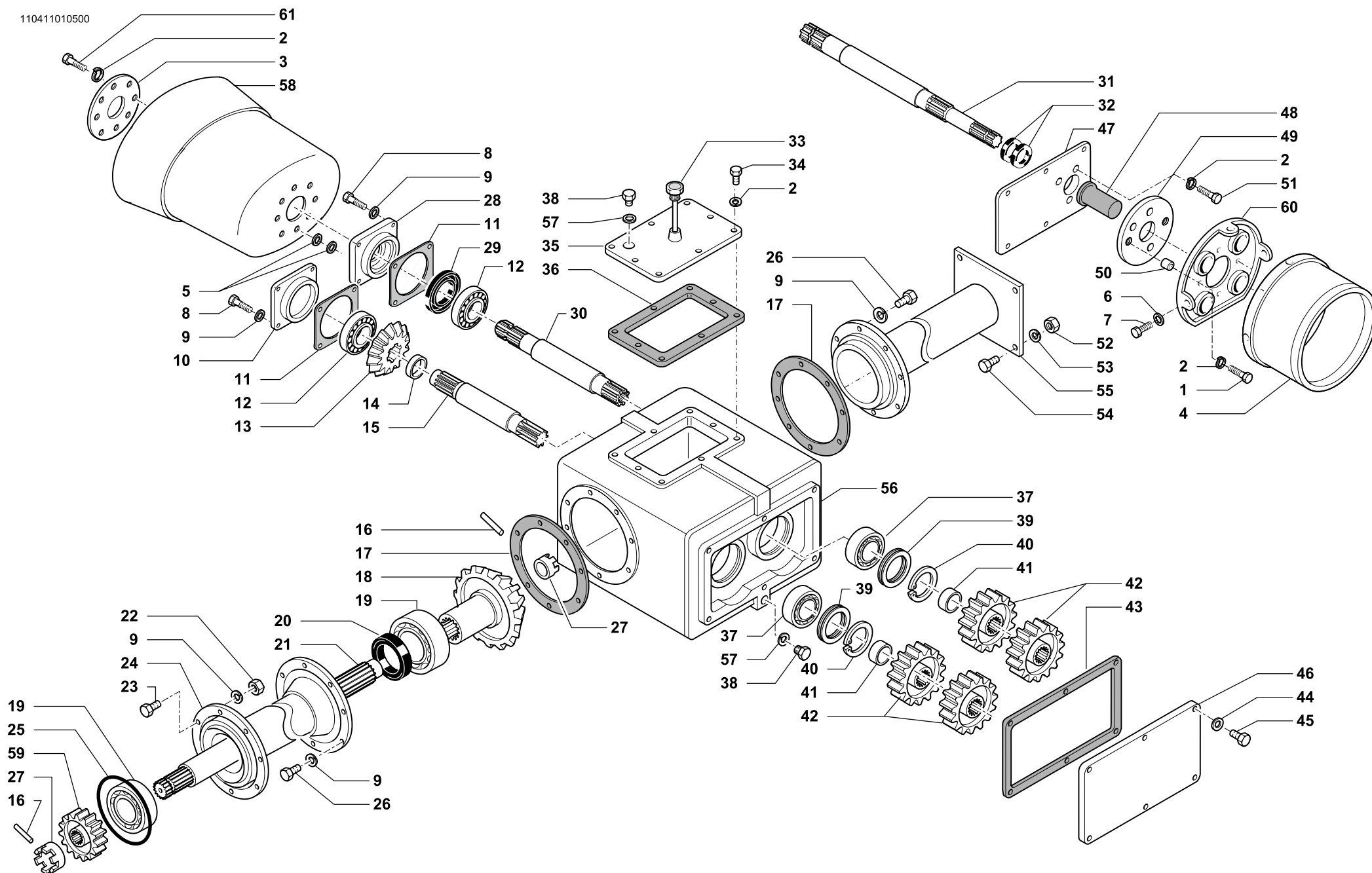
2 SPEED GEARBOX 540/1000 rpm
