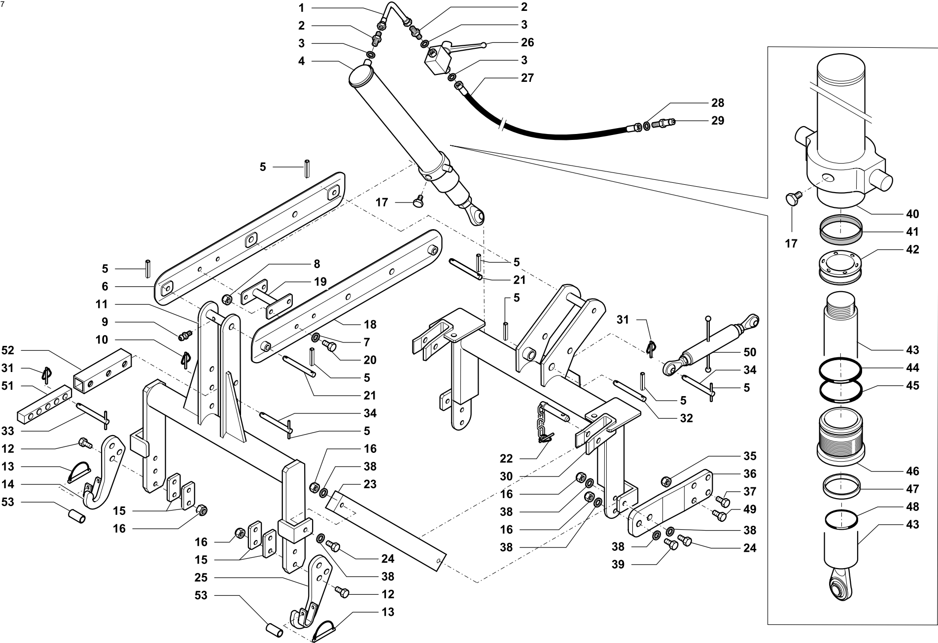
HYDRAULIC SEEDING MACHINE HITCH
