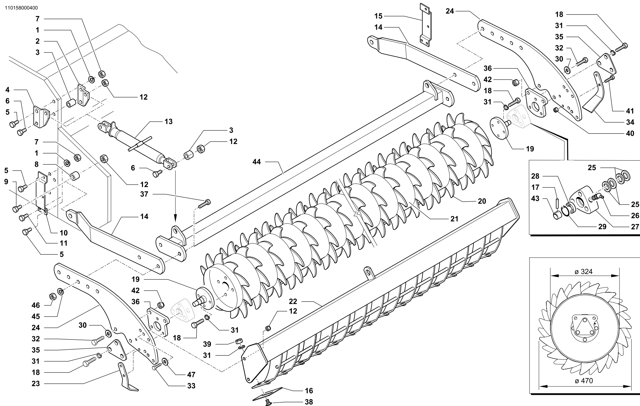
PACKER ROLLER Ø 470
