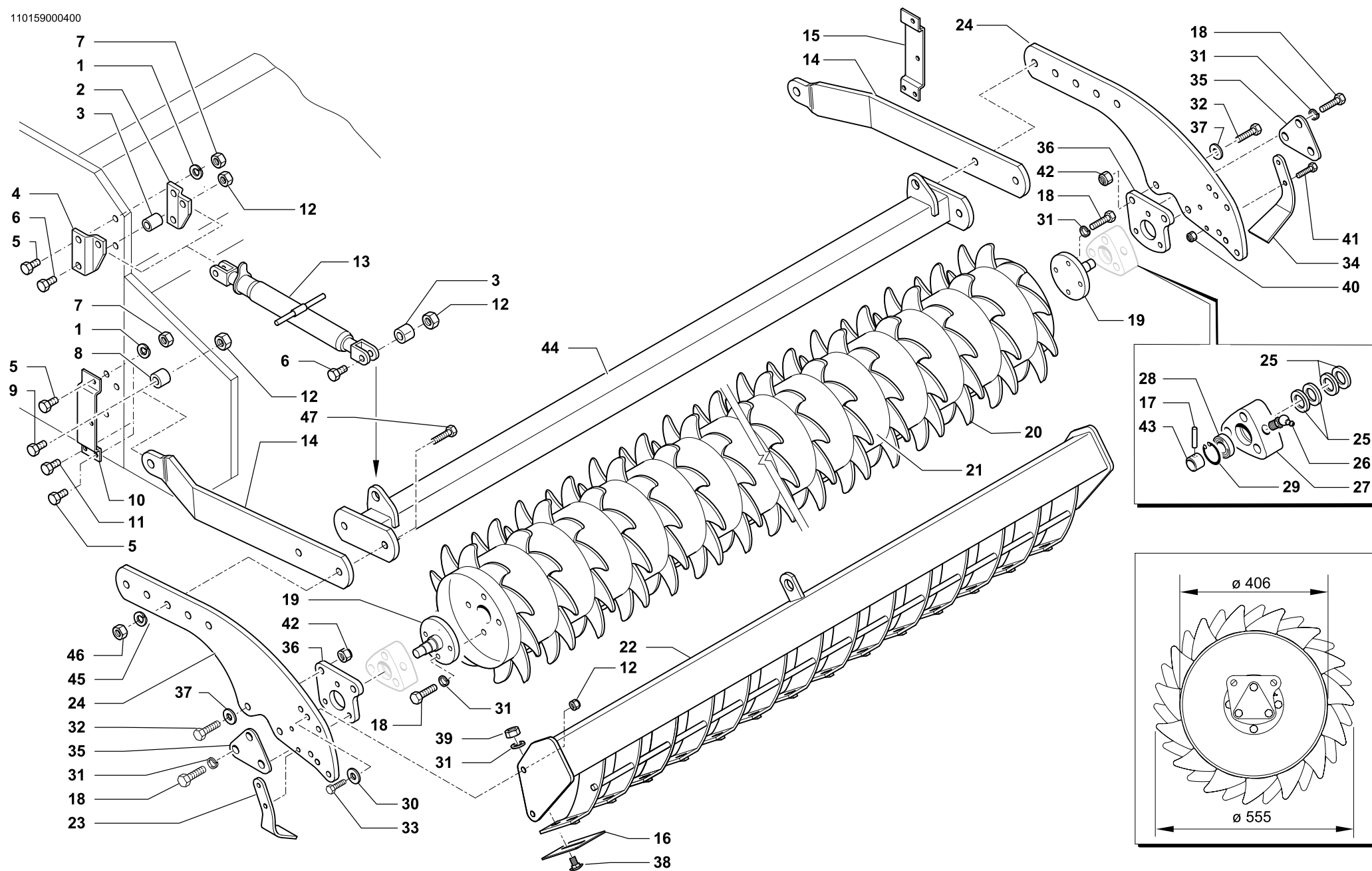
PACKER ROLLER Ø 555
