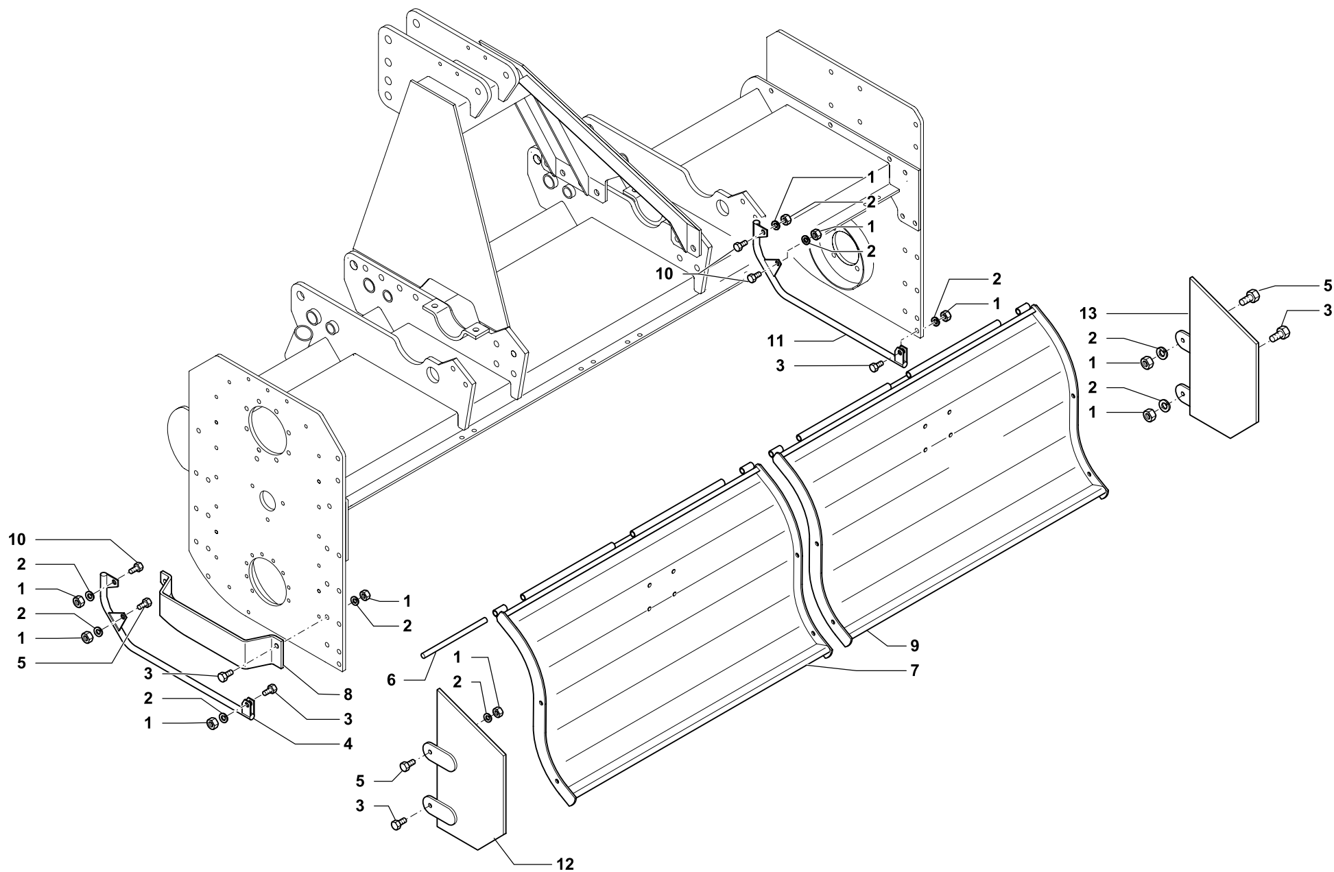
FRAME GROUP (VERSION WITH ROLLER/WHEELS)
